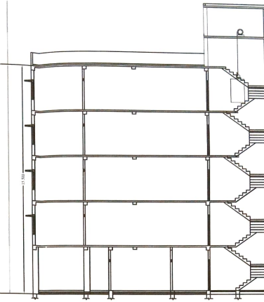
SECTION AT "C-D" SCALE- 1:100
