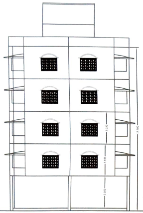
ELEVATION SCALE- 1:100
