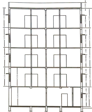
SECTION AT "A-B" SCALE- 1:100
